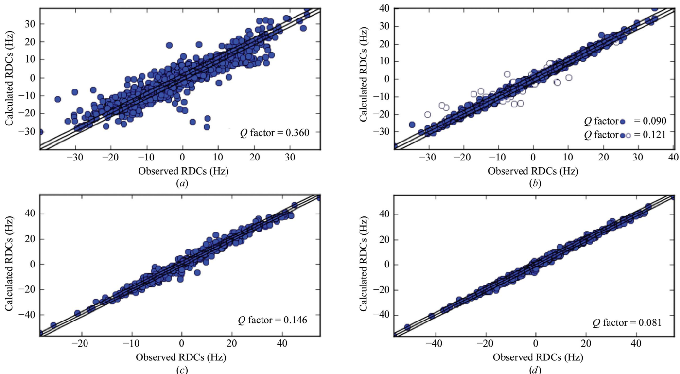
Figure 4 Calculated versus observed RDCs for Ub ( a , b ) and GB3 ( c , d ) before ( a , c ) and after ( b , d ) joint refinement against RDCs and X-ray data. The empty symbols in ( b ) show the values for residues 8 and 72.
